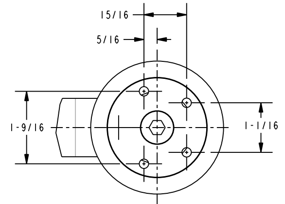
DETAIL A SCALE 0.500 WALL MOUNT
