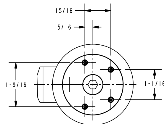
DETAIL A SCALE 0.500 WALL MOUNT
