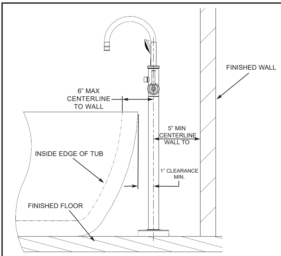
Figure 1 Installation Clearances
