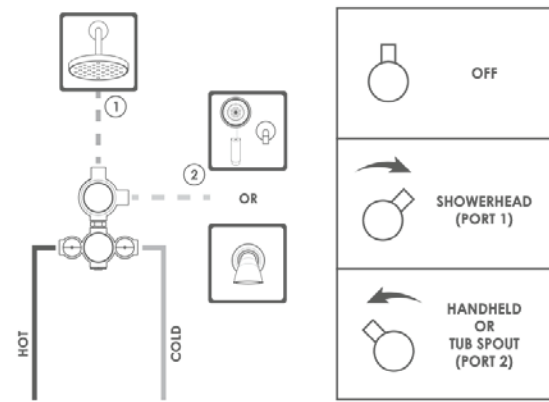
I-744 THERMOSTATIC VALVE
