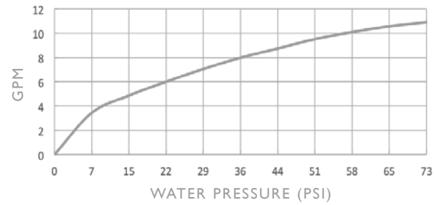
I-741 THERMOSTATIC VALVE
