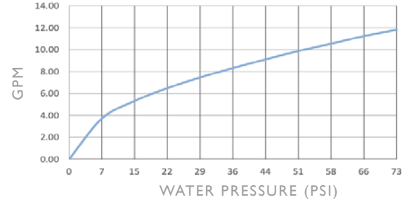
I-742 THERMOSTATIC VALVE
